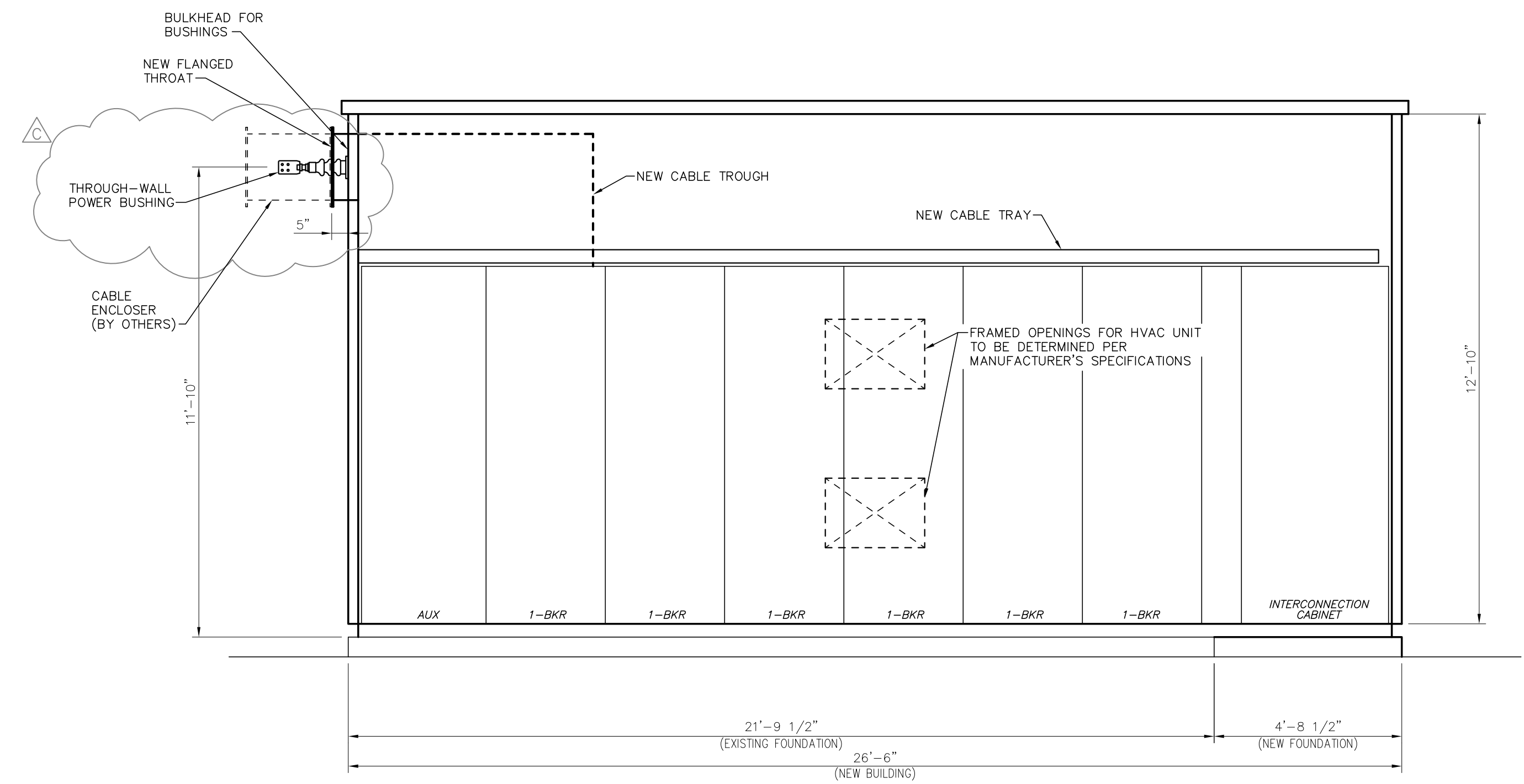
NEW MCC BUILDING SECTION A-A SCALE: 3/8"=1'-0"
